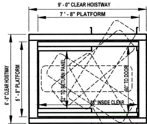
RIGHT HAND SHOWN, LEFT HAND OPPOSITE 2800 88" w BY 52" D FRONT AND REAR OPENING
