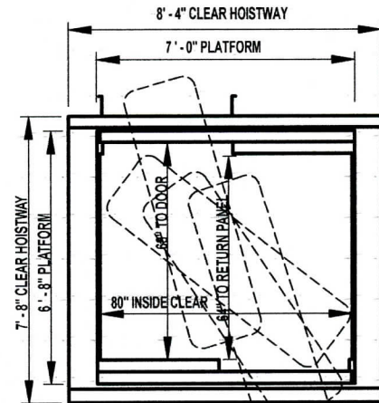
RIGHT HAND SHOWN, LEFT HAND OPPOSITE 3500 80" w BY 64" D FRONT AND REAR OPENING
