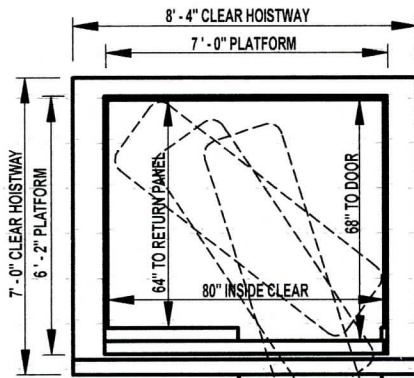
RIGHT HAND SHOWN, LEFT HAND OPPOSITE 3500 80" w BY 64" d FRONT OPENING
