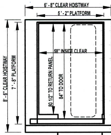
RIGHT HAND SHOWN, LEFT HAND OPPOSITE 2800 58" w BY 80.5d FRONT OPENING
