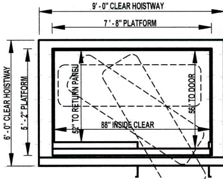
RIGHT HAND SHOWN, LEFT HAND OPPOSITE 2800 88w BY 52d FRONT OPENING
